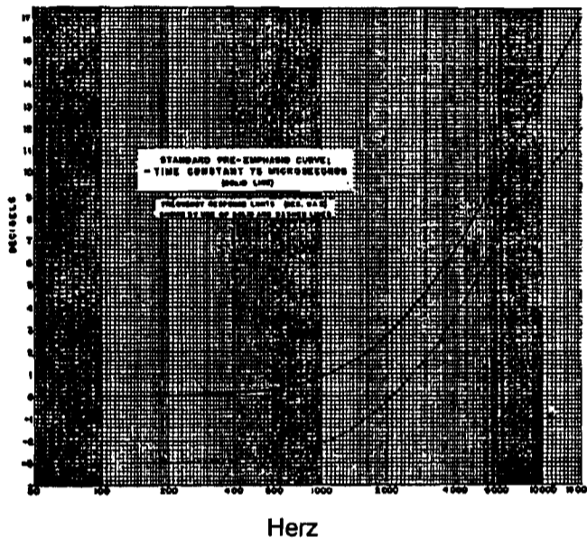
Figura 4.2. Curva de preénfasis Federal Communications Commission § 73.333
